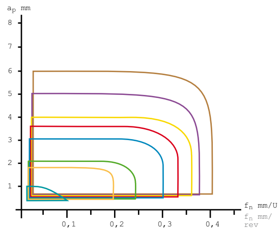
Plandrehen 2,25D Face turning 2,25D
